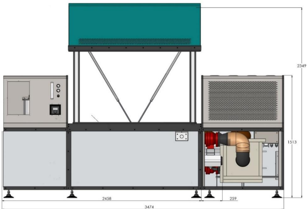
Figure 7 Mechanical dimensions
